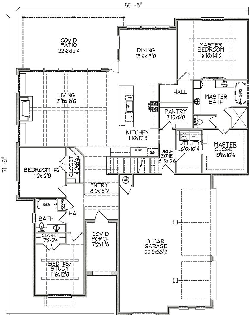
A Lower Level Floor Plan
